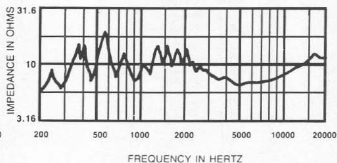
FIGURE 7 Impedance Response — HP9040 Horn 8-Ohm Driver
