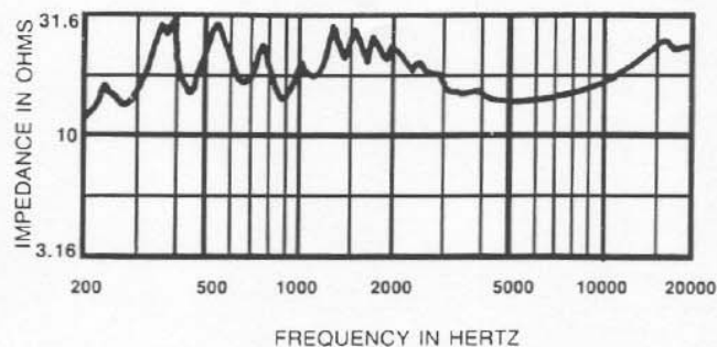
FIGURE 9 Impedance Response — HP9040 Horn 16-Ohm Driver
