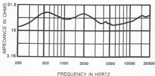
FIGURE 8 Impedance Response — 2-Inch Plane-Wave Tube 16-Ohm Driver
