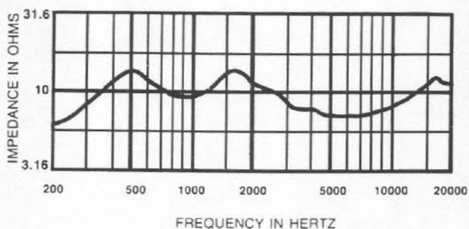
FIGURE 6 Impedance Response — 2-Inch Plane-Wave Tube 8-Ohm Driver
