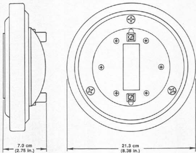
FIGURE 2 Dimensions
